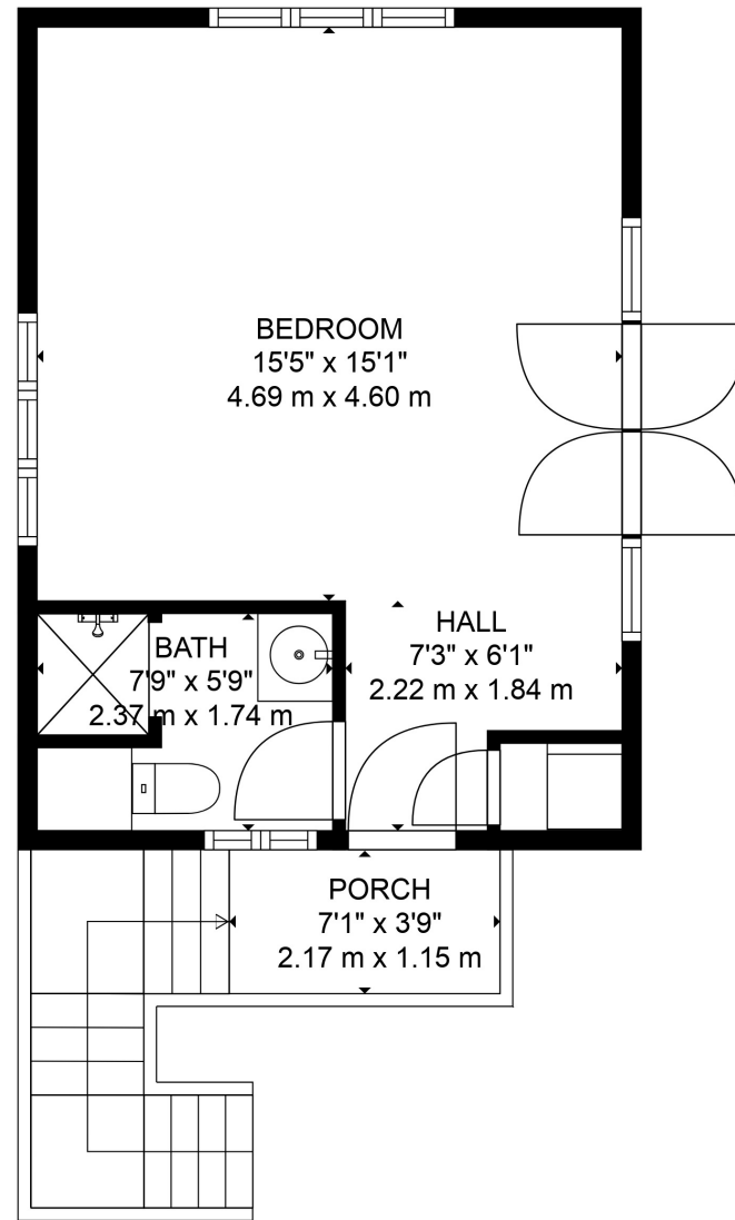
FLOOR 2
