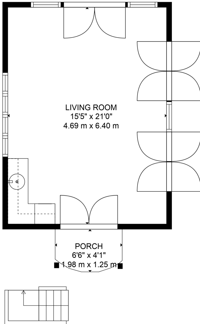
FLOOR 1
